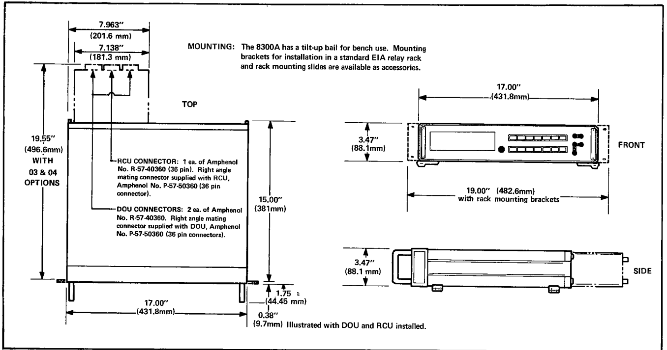
Figure 1-1. OUTLINE DRAWING
